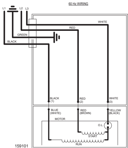
WIRING DIAGRAM FOR MODELS "E7021 w/REMOTE CAPACITOR" All Revisions 10/24 thru Current
