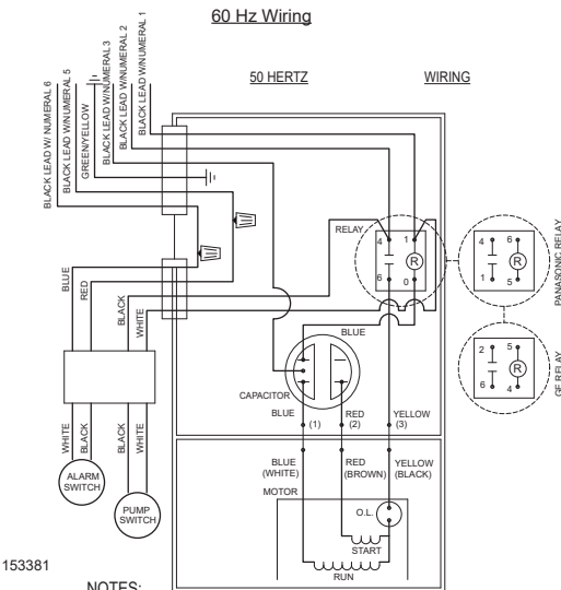
WIRING DIAGRAM FOR MODEL "RWD7021" & "RWH7021" All revisions thru Current
