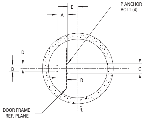
SIMPLEX DIMENSIONAL CHART
