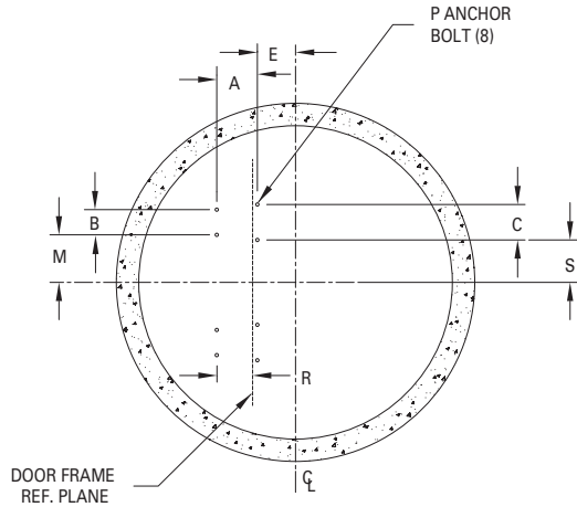
DUPLEX DIMENSIONAL CHART
