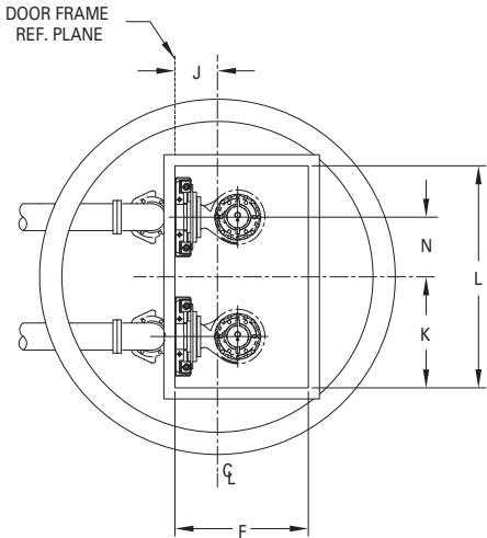
DUPLEX DIMENSIONAL CHART
