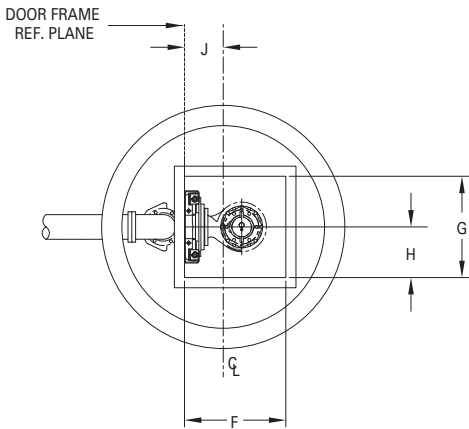
SIMPLEX DIMENSIONAL CHART
