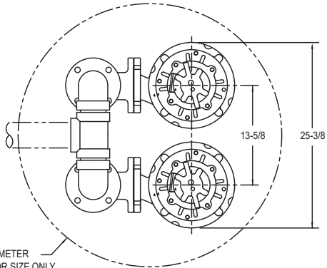
DUPLEX INSTALLATION
