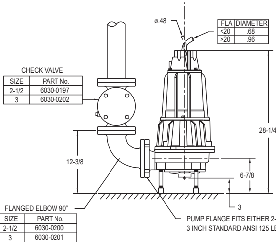
SIMPLEX INSTALLATION
