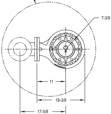
SIMPLEX INSTALLATION
