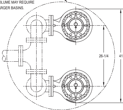
DUPLEX INSTALLATION
