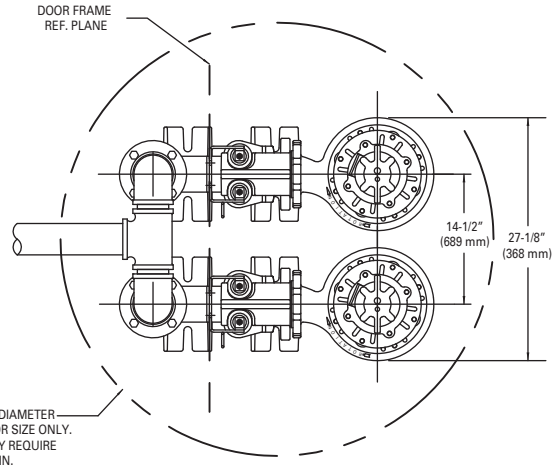
DUPLX INSTALLATION DIMENSIONS BASED ON STD. ANSI FITTING SIZES CHECK VALVES REQUIRED, NOT SHOWN FOR CLARITY ALL DIMENSIONS IN INCHES UNLESS OTHERWISE NOTED
