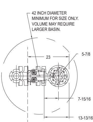
SIMPLEX INSTALLATION
