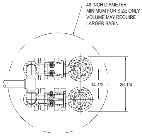
DUPLEX INSTALLATION
