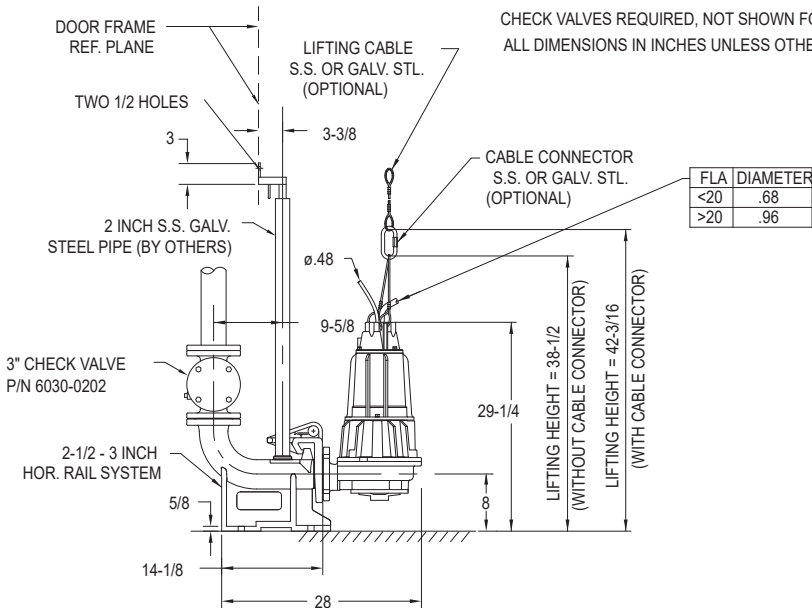
SIMPLEX INSTALLATION
