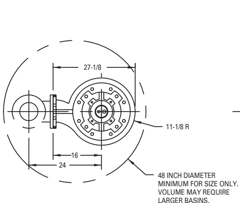
SIMPLEX INSTALLATION
