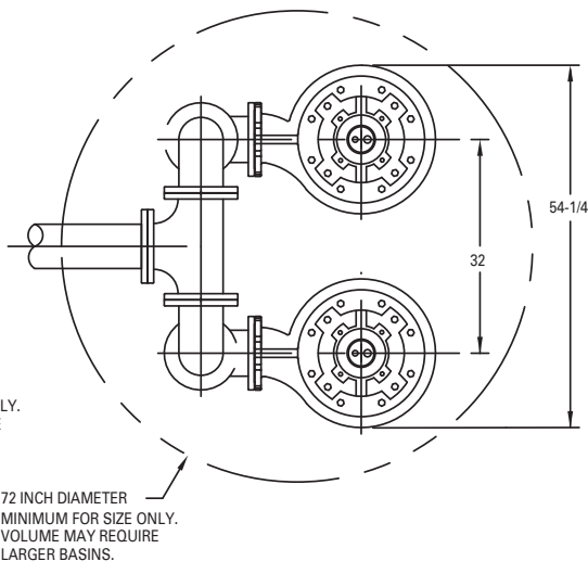
DUPLEX INSTALLATION DIMENSIONS BASED ON STD. ANSI FITTING SIZES CHECK VALVES REQUIRED, NOT SHOWN FOR CLARITY
