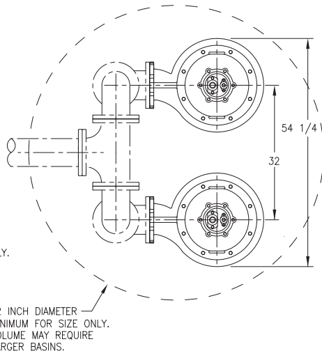
DUPLEX INSTALLATION DIMENSIONS BASED ON STD. ANSI FITTING SIZES CHECK VALVES REQUIRED, NOT SHOWN FOR CLARITY
