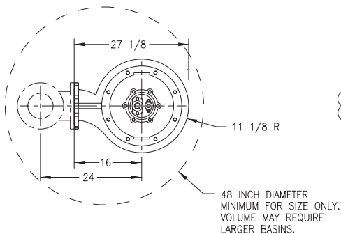
SIMPLEX INSTALLATION
