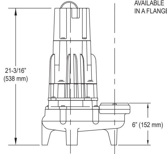
Double Seal, 290 Series
