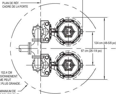
INSTALLATION DUPLEX
