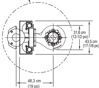
INSTALLATION SIMPLE
