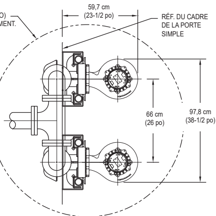
INSTALLATION DUPLEX
