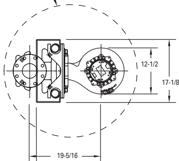
SIMPLEX INSTALLATION
