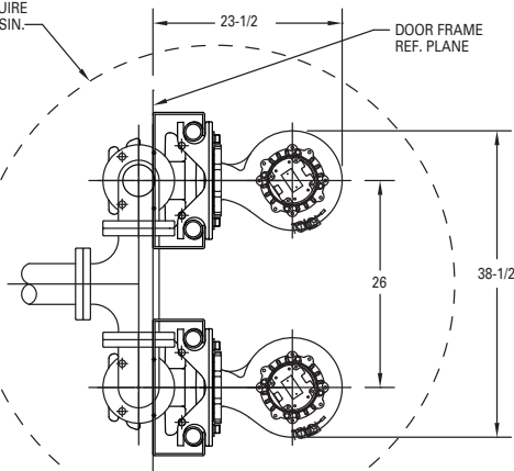
DUPLEX INSTALLATION
