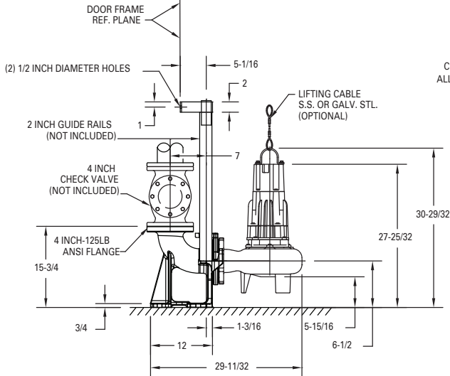
SIMPLEX INSTALLATION
