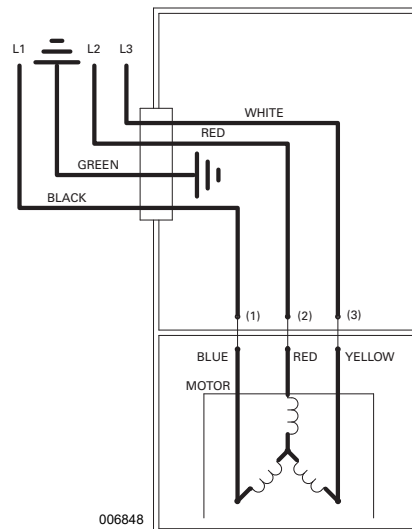
WIRING DIAGRAM FOR MODELS "J7009", "F7009", "G7009", and "BA7009" All Revisions 09/17 thru Current
